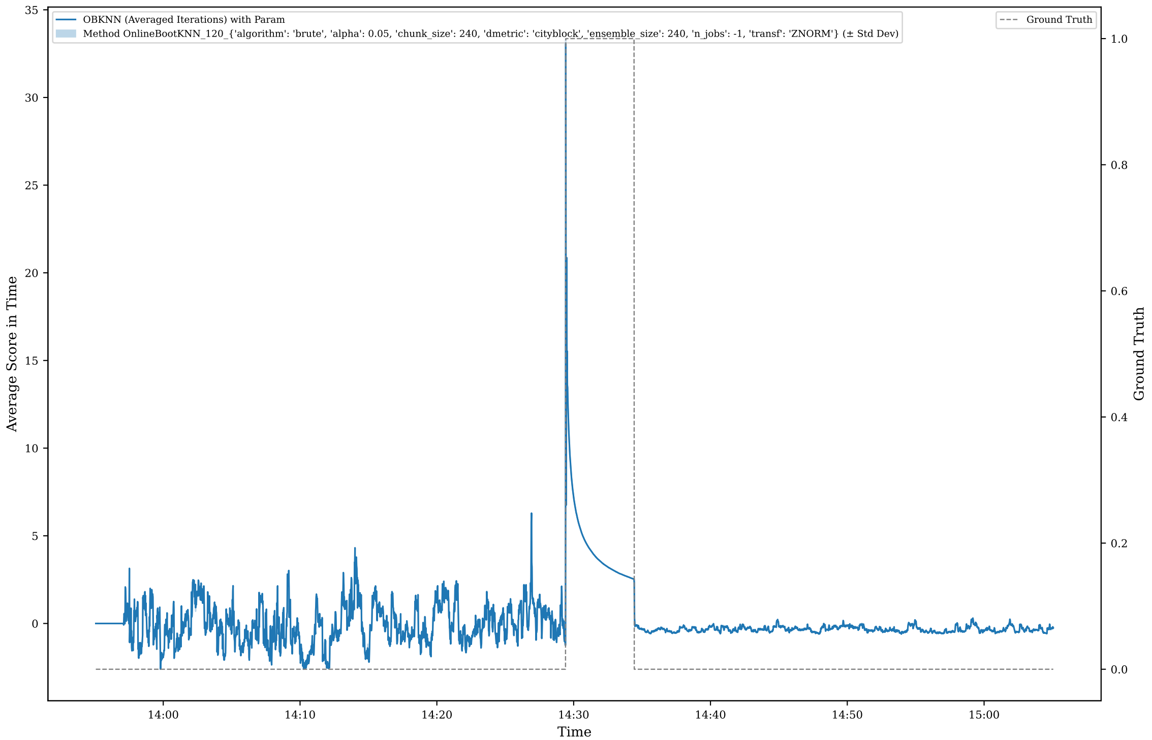
Method OBKNN Score for Scenario A2
